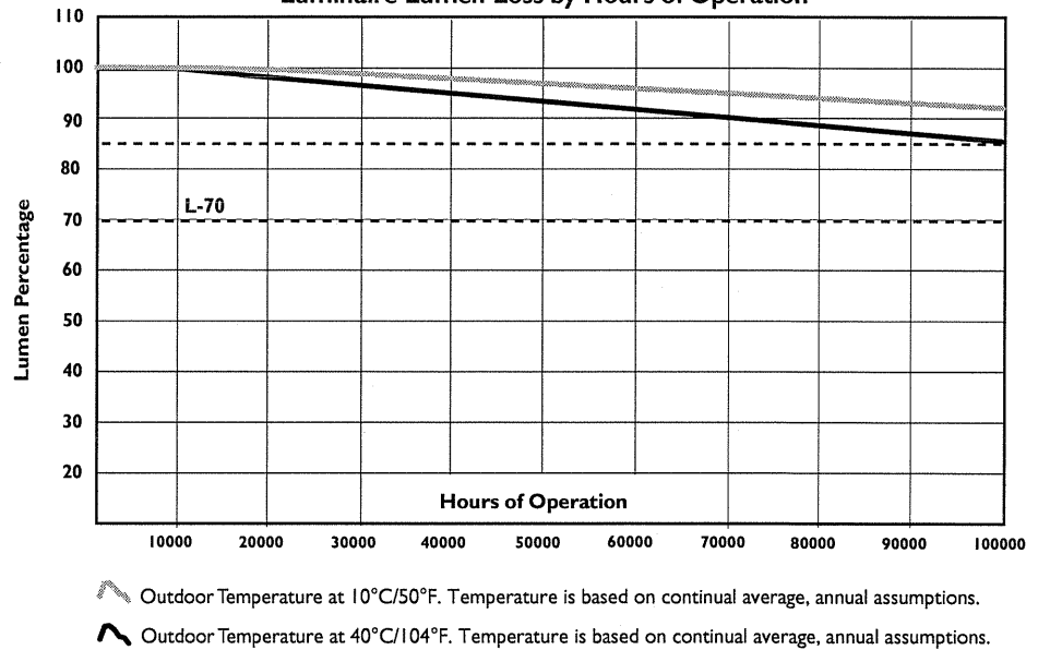
Luminaire Lumen Loss by Hours of Operation
