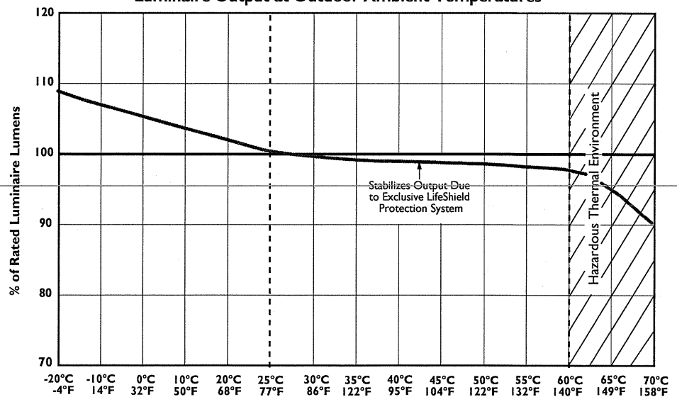
Luminaire Output at Outdoor Ambient Temperatures
