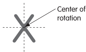
The letter 'X' shows line and rotational symmetry.
