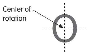
The letter 'O' shows line and rotational symmetry.
