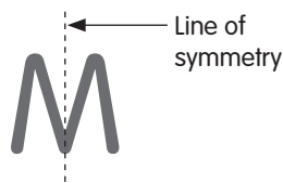
The letter 'M' shows line symmetry.
