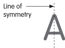
The letter 'A' shows line symmetry.
